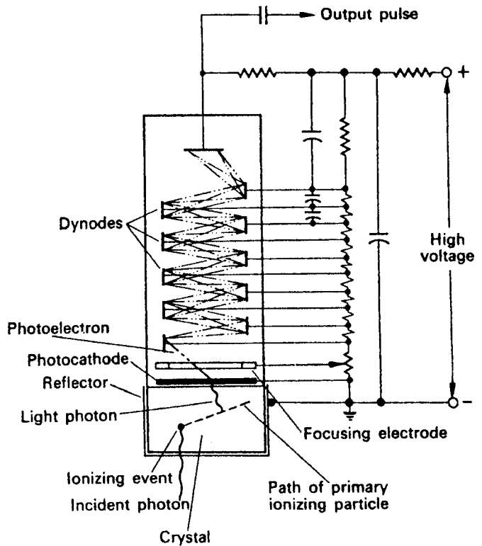
Figure 9-9. Schematic representation of the sequence of events in the detection of a gamma-ray photon by a scintillation counter. An average of about four electrons are knocked out of a dynode by an incident electron.
