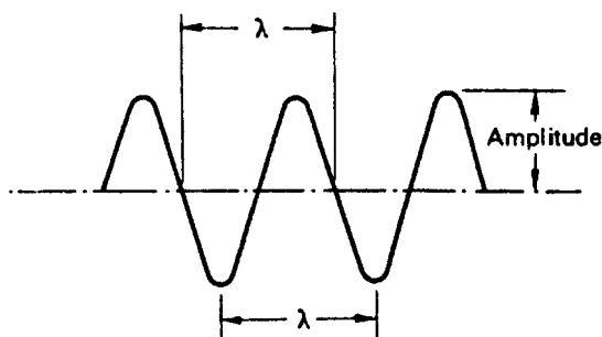
Figure 2-11. Graphical representation of a wave.
