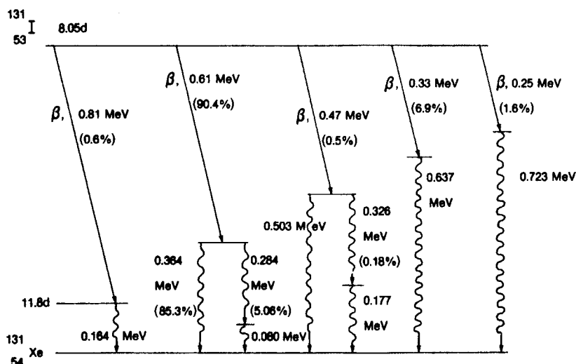
Figure 4-7. Iodine-131 transformation (decay) scheme.
