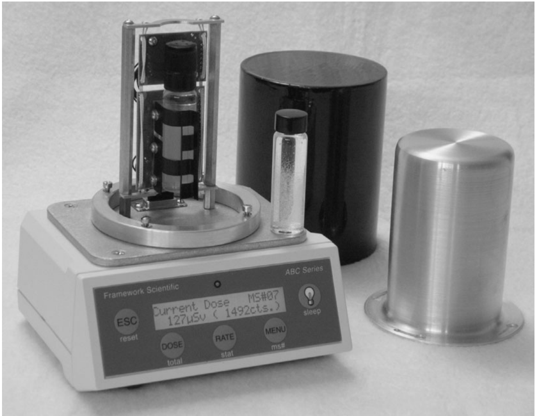
Figure 9-36. Photograph of a superheated emulsion vial and acoustical bubble counter. The lead cylinder in the background is used to extend the response to over 1 GeV. (Courtesy of FrameSci.com.)
